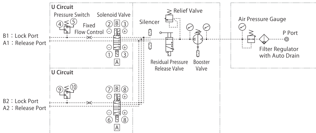
Circuit Symbol : UU
